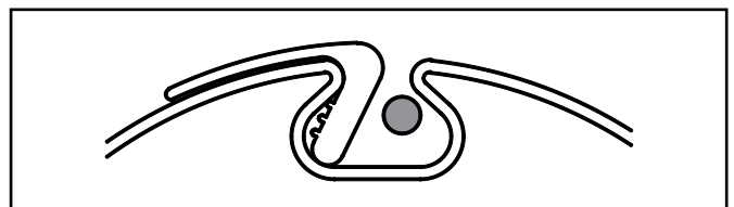
Fig. 2 : "Clip-on clip-off" profiel
