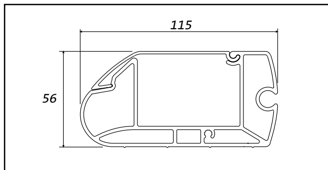
Fig. 4 : Front rail
