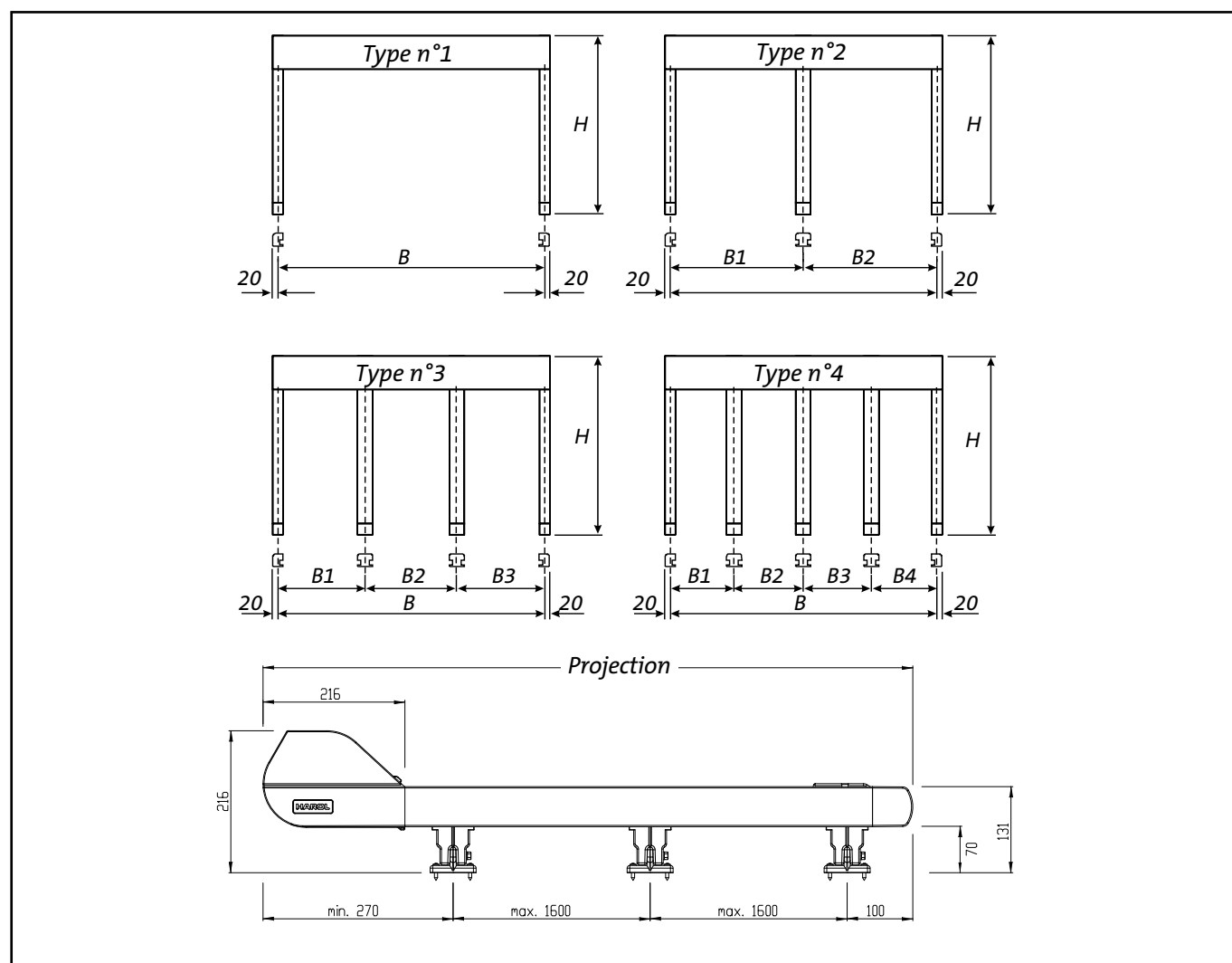
Fig. 14 : Measuring and assembly
