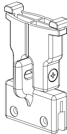
Fig. 8 : Standard aluminium support
