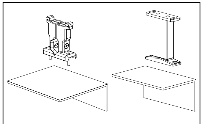
Fig. 10 : Mounting against the wall
