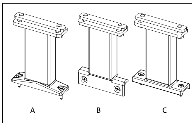
Fig. 11 : Higher attachment points
