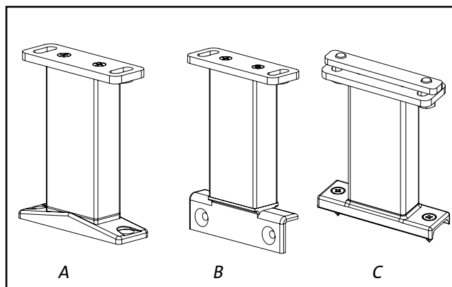
Fig. 9 : Higher attachment point
