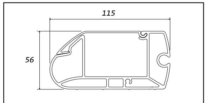
Fig. 4 : Front rail
