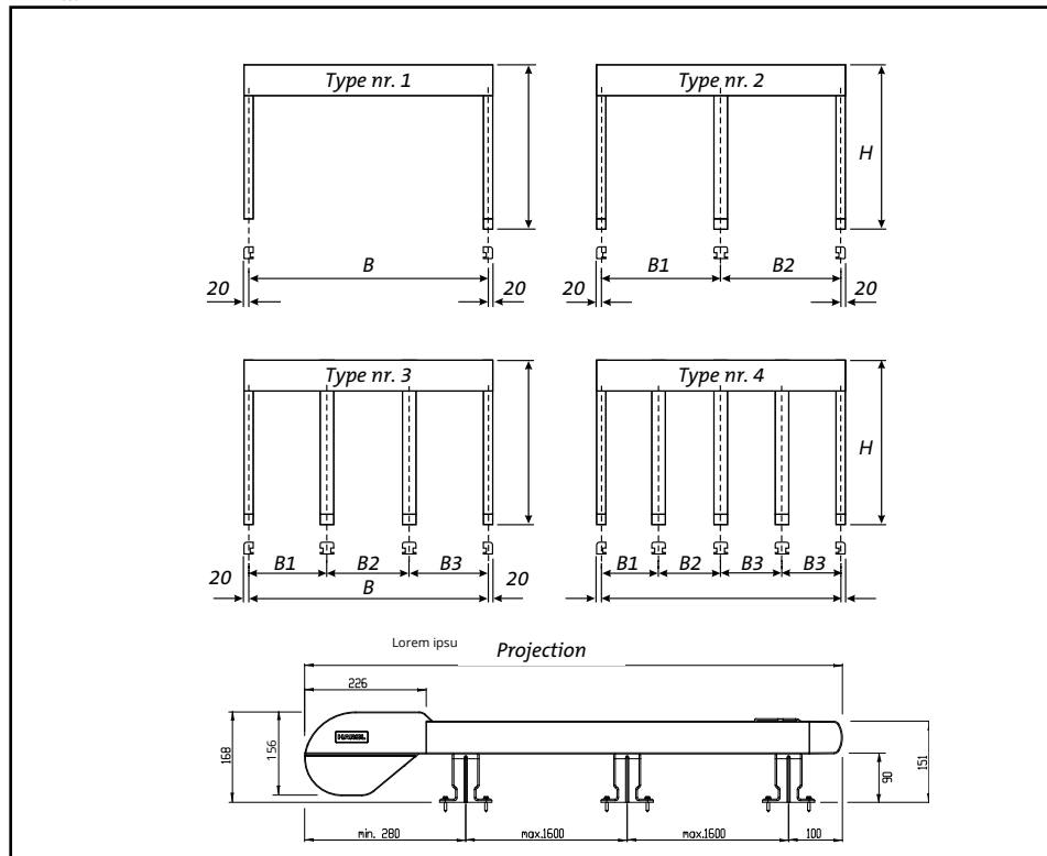
Fig. 16 : Measuring and assembly
