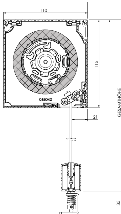
Coolscreen 7 110x115
