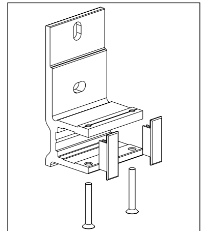
Fig. 9 : Wall support
