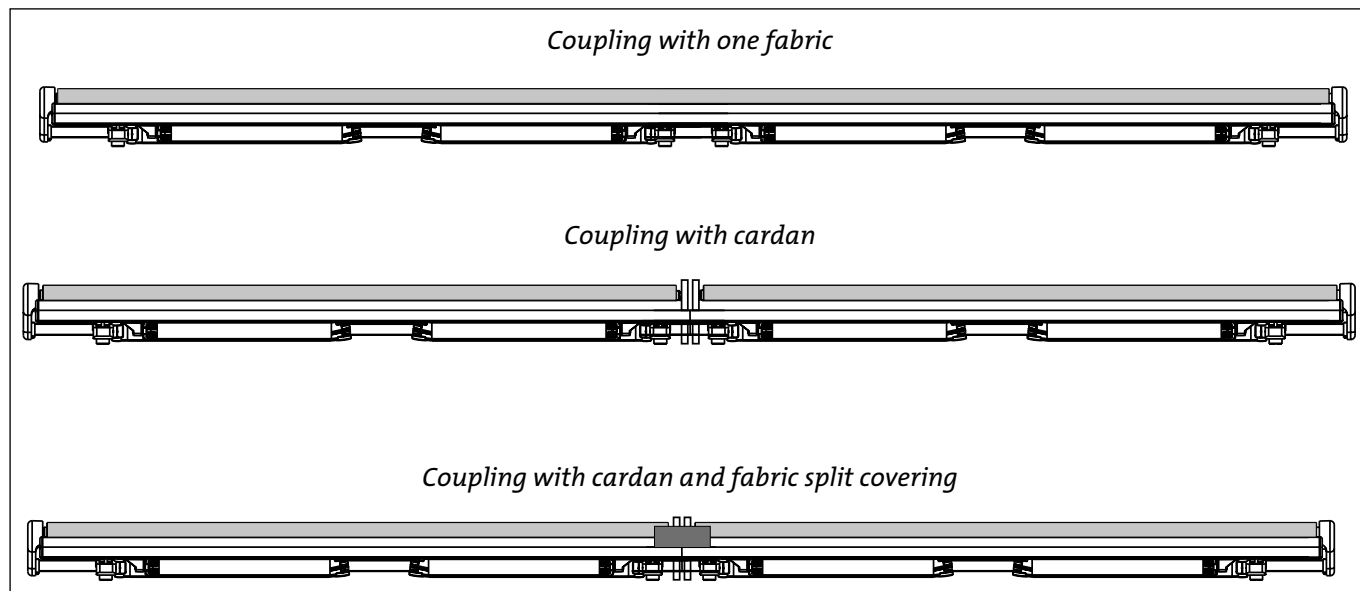
Fig. 14 : Coupling possibilities
