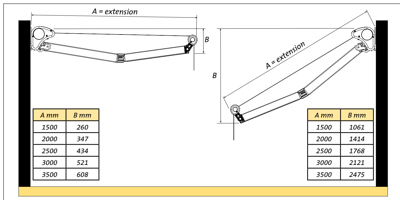
Fig. 17 : Minimum and maximum angles
