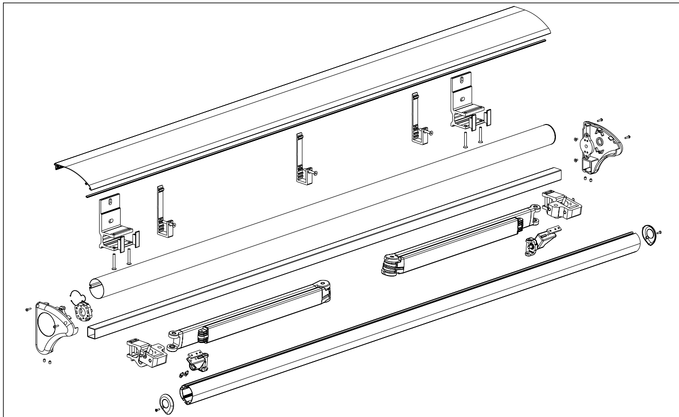
Fig. 2 : Exploded view PR220
