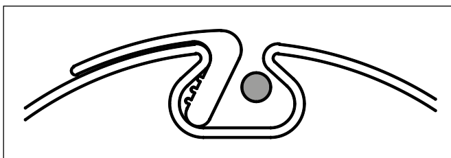
Fig. 1 : "Clip On - Clip Off" profiel
