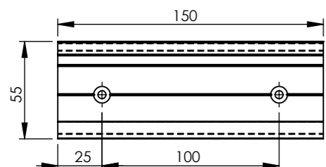
BRACKET WITH PADDING
