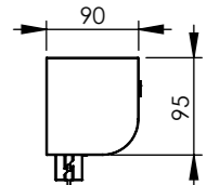
SIDE VIEW right
