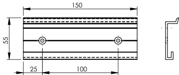
BRACKET WITH PADDING
