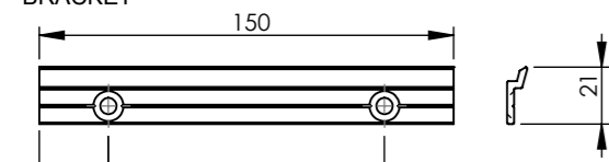
BRACKET
