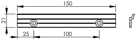
BRACKET
