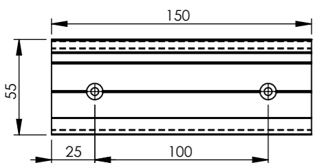
BRACKET WITH PADDING
