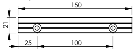
BRACKET
